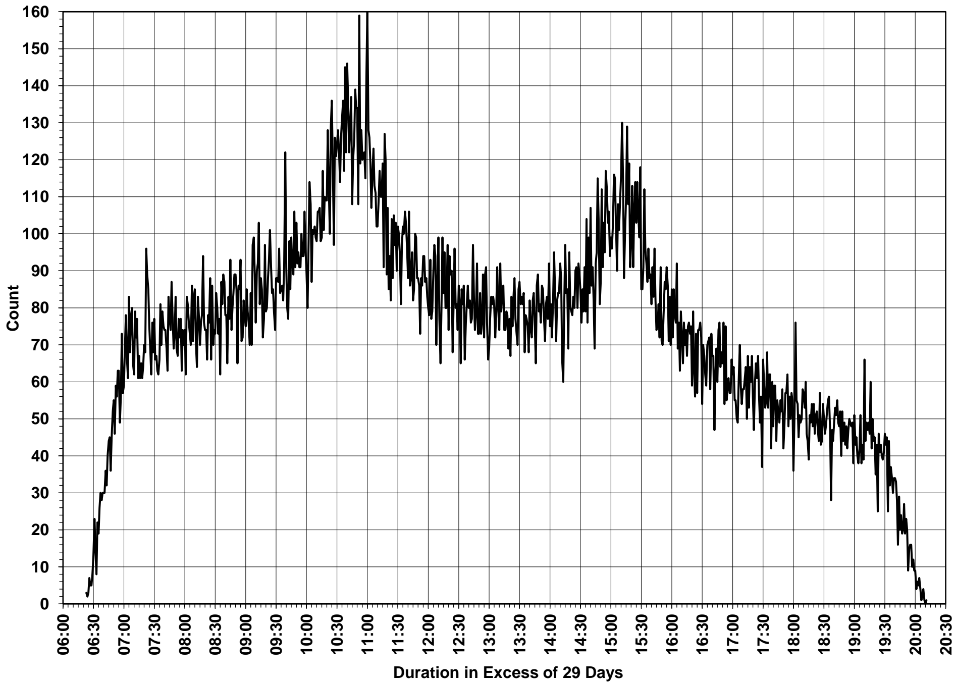
Lunar Cycle Durations (rounded to the minute) from 2000 BC through 3000 AD
