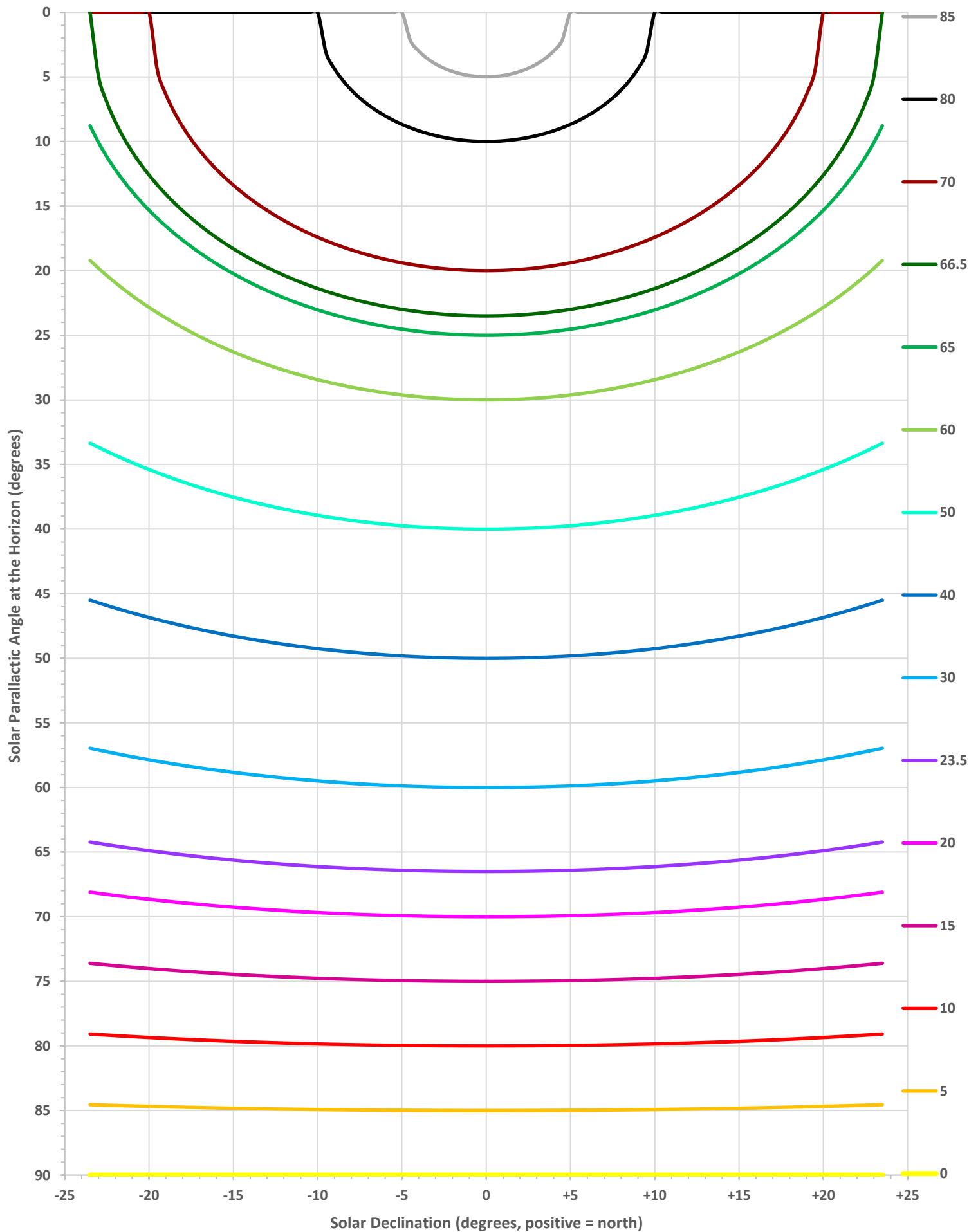
Variation of the Horizon Solar Parallactic Angle for Selected Latitudes
